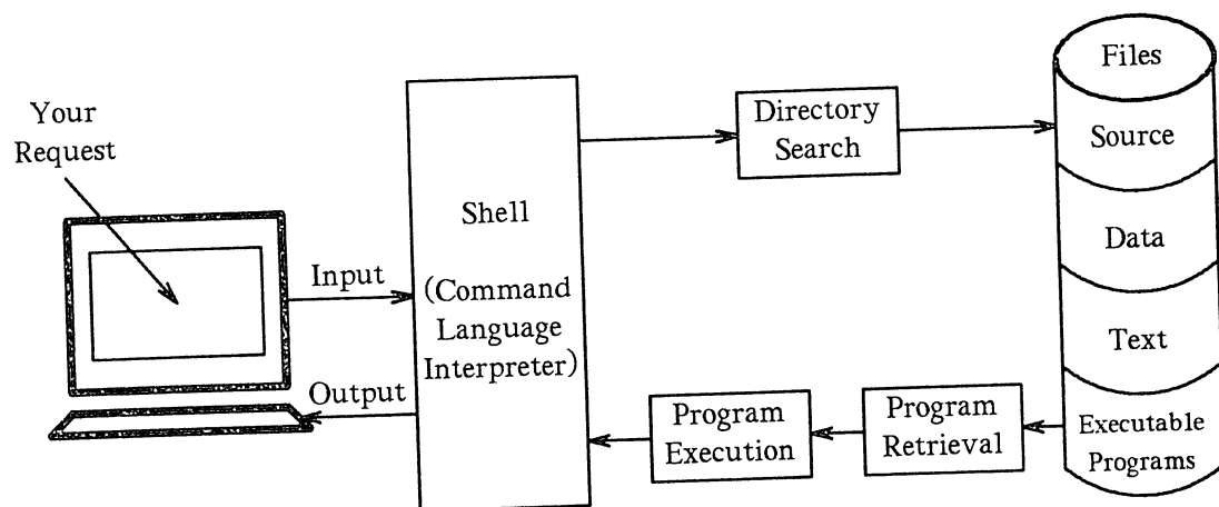
Figure 2-5. Execution of a GENIX V.3 System Command
