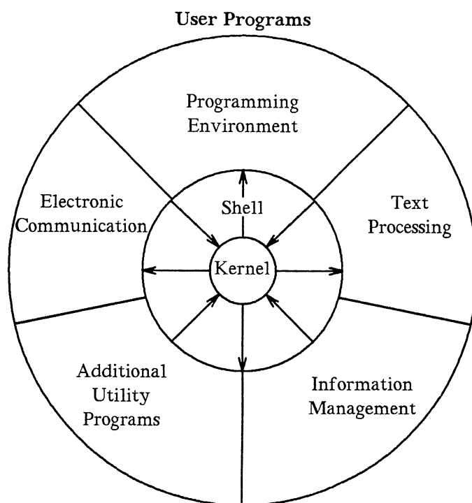
Figure 2-1. Model of the GENIX V.3 System
